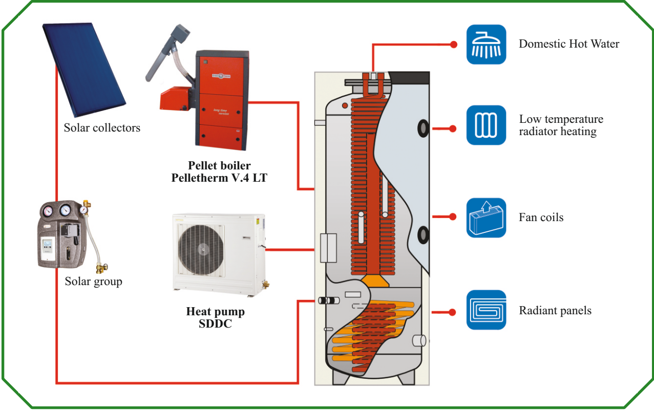
Principle scheme of a Smart Hybrid System for heating with air-water heat pump, heating pellet boiler, solar collector and insulation tank
